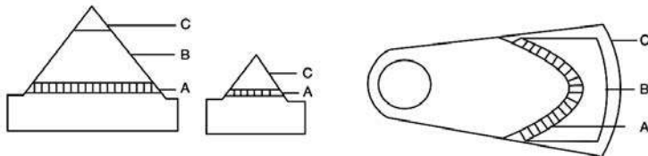
A- Buffer Welding with ELOX B 307 B- Build-Up with ELHARD 14 Mn C- Hardfacing with ELHARD 600
